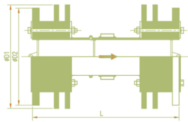
BI-DIRECTIONAL MAGNETIC PIG 4" TO 12" PIGS ASSEMBLY
